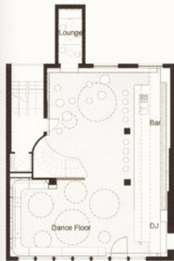
2F PLAN
