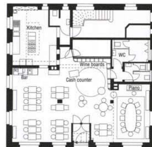
▲ BELLA ITALIA PLAN S=1:300
